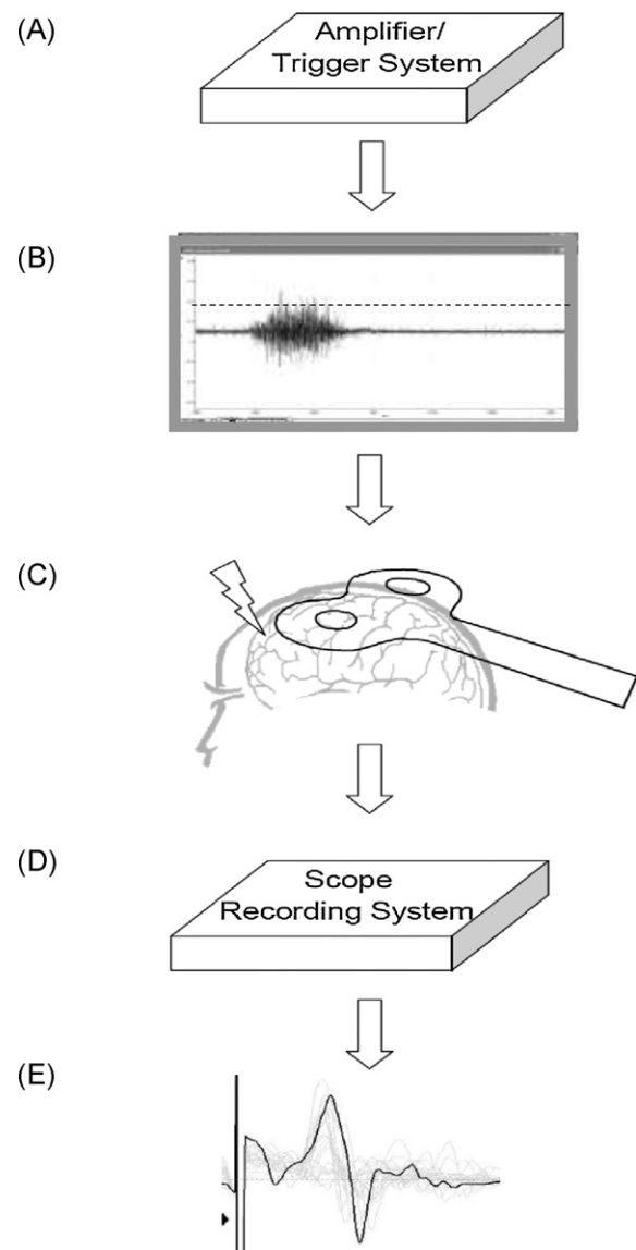
Fig. 1. Illustration of triggering system. An amplifier and custom-made triggering system (A) monitor surface electromyographic activity during muscle activation (B). Upon breach of a pre-set threshold, a TTL pulse is generated to trigger the magnetic stimulator (C) which subsequently triggers the recording of a 200-ms sweep in the Scope recording software (D). (E) Displays the averaged MEP signal across 15 trials of one research participant.
